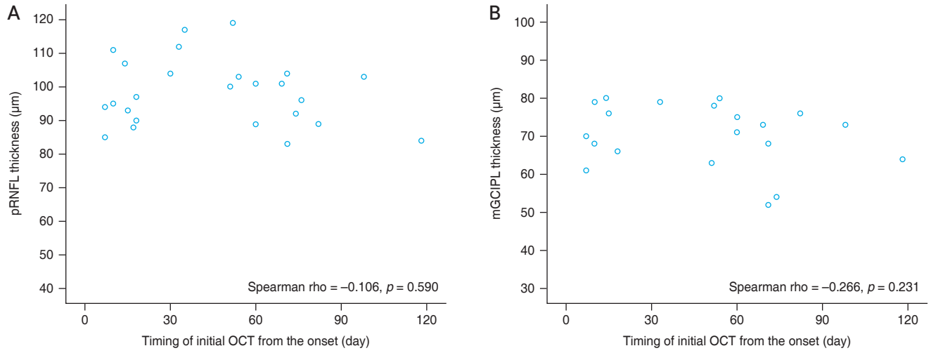
Supplementary Fig. 1. Correlation between the timing of initial optical coherence tomography (OCT) with the initial thickness of (A) peripapillary retinal nerve fiber layer (pRNFL) and (B) macular ganglion cell-inner plexiform layer (mGCIPL).
